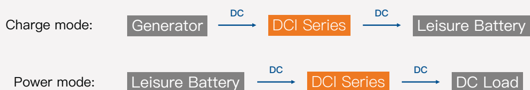
Wiring diagram
